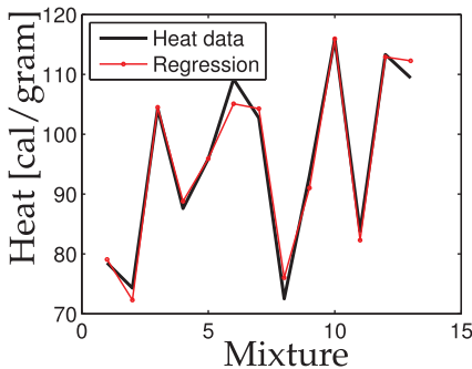
Figure 1.10 Heat data for cement mixtures containing four basic ingredients.
