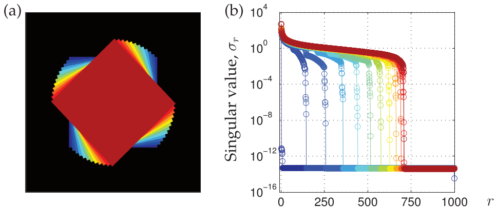
Figure 1.26 A data matrix consisting of zeros with a square sub-block of ones at various rotations (a), and the corresponding SVD spectrum, \text{diag}(\mathbf{S}) , (b).
