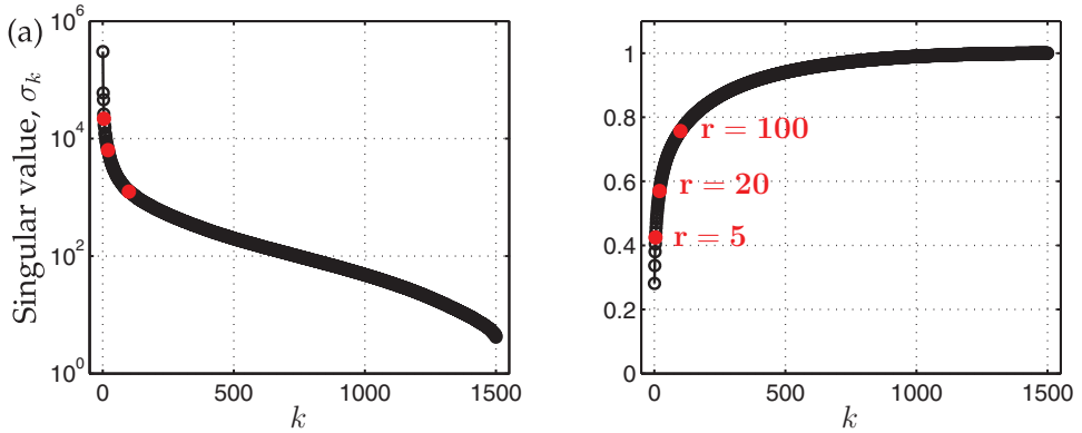
Figure 1.4 (a) Singular values \sigma_k . (b) Cumulative energy in the first k modes.
