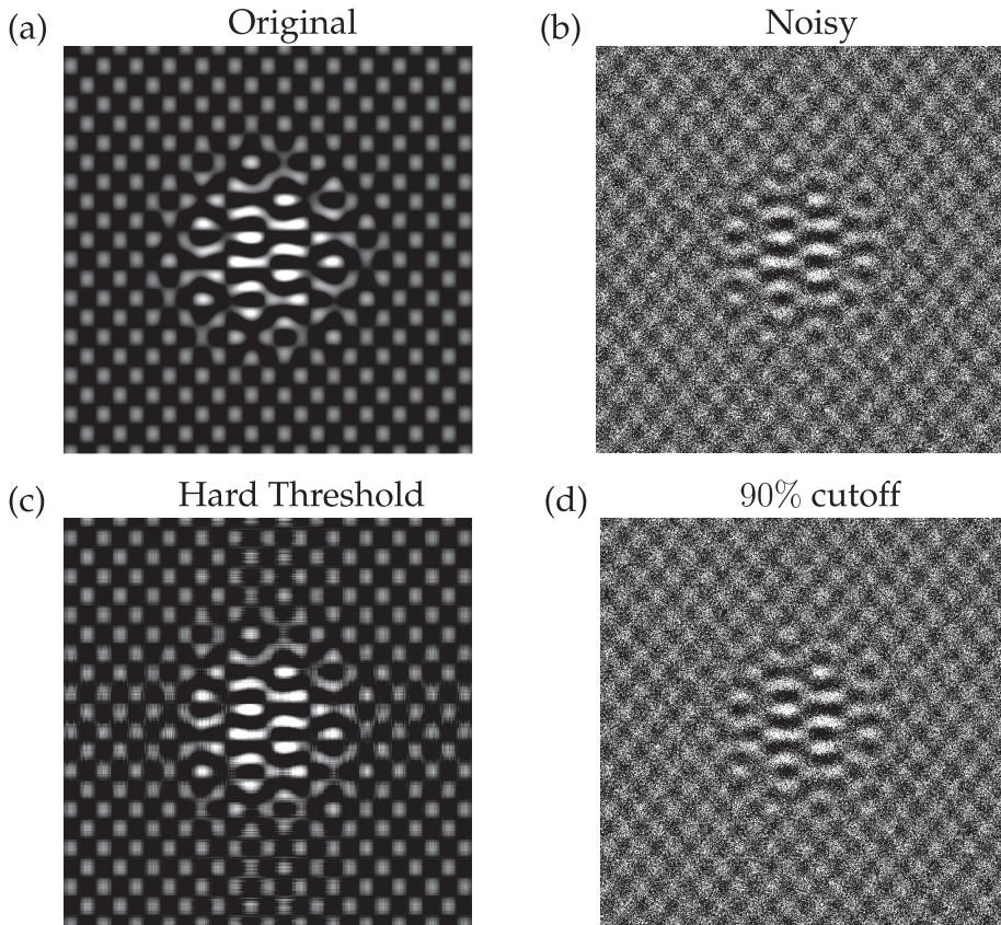
Figure 1.22 Underlying rank 2 matrix (a), matrix with noise (b), clean matrix after optimal hard threshold (4/\sqrt{3})\sqrt{n}\sigma (c), and truncation based on 90% energy (d).
