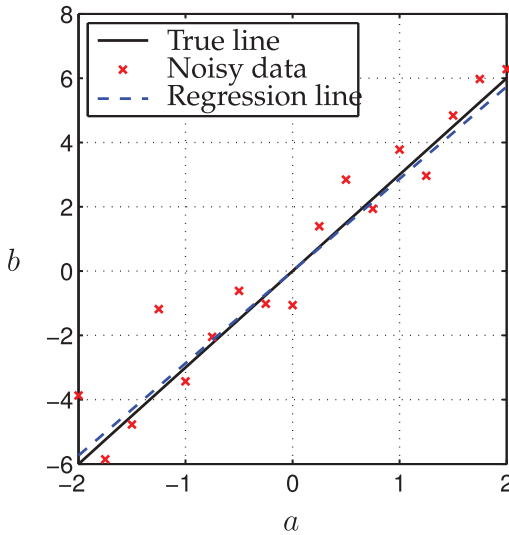
Figure 1.9 Illustration of linear regression using noisy data.
