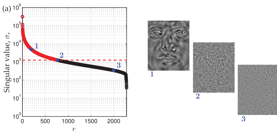
Figure 1.24 Hard thresholding for eigenfaces example.
