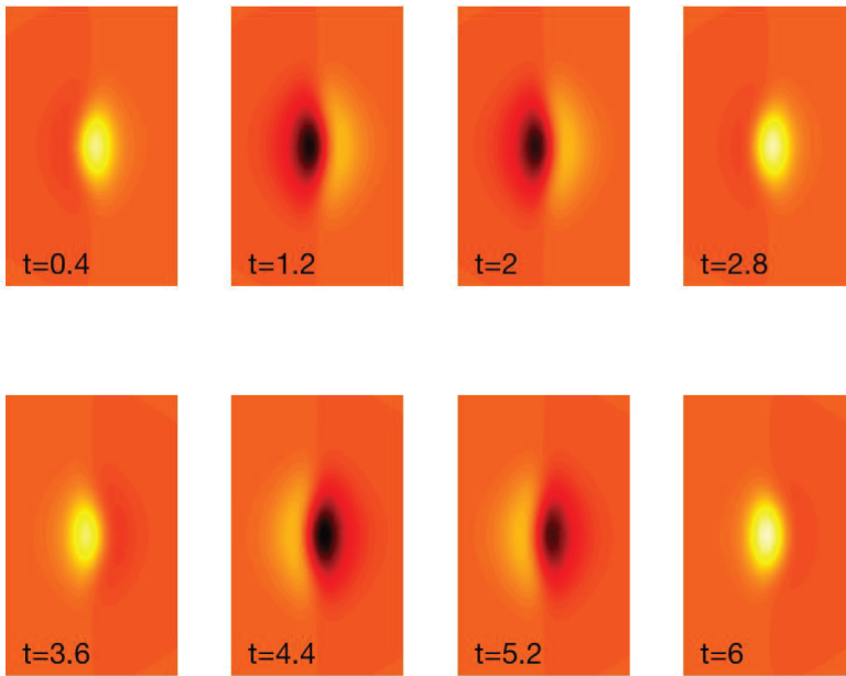
Figure 1.30 Example N -way array data set created from the function (1.45). The data matrix is \mathbf{A} \in \mathbb{R}^{121 \times 101 \times 315} . A CP tensor decomposition can be used to extract the two underlying structures that produced the data.
