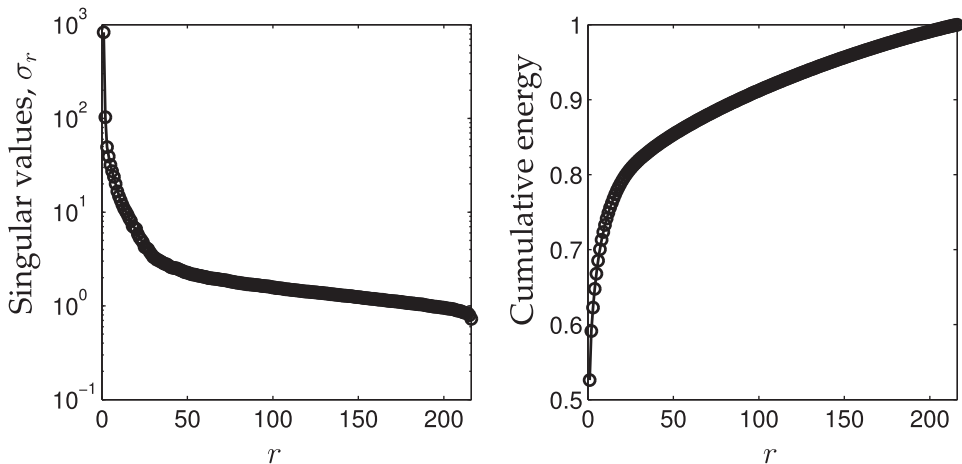
Figure 1.14 Singular values for the Ovarian cancer data.
