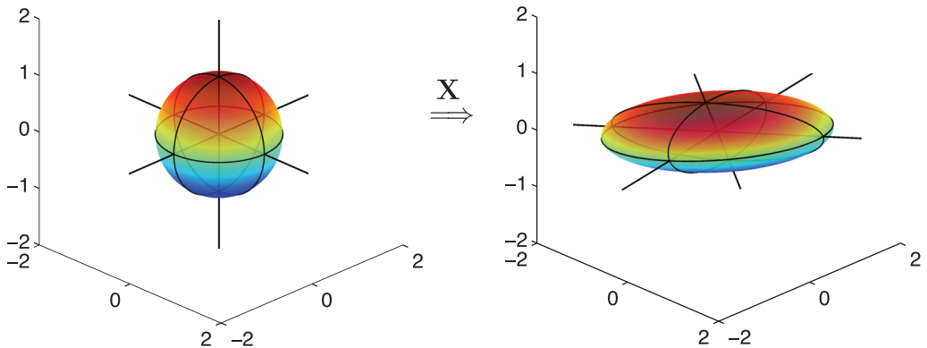
Figure 1.8 Geometric illustration of the SVD as a mapping from a sphere in \mathbb{R}^n to an ellipsoid in \mathbb{R}^m .
