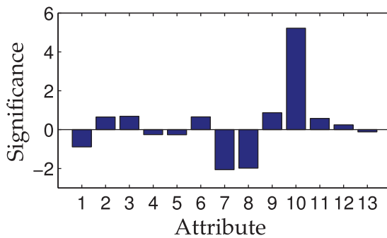
Figure 1.12 Significance of various attributes in the regression.
