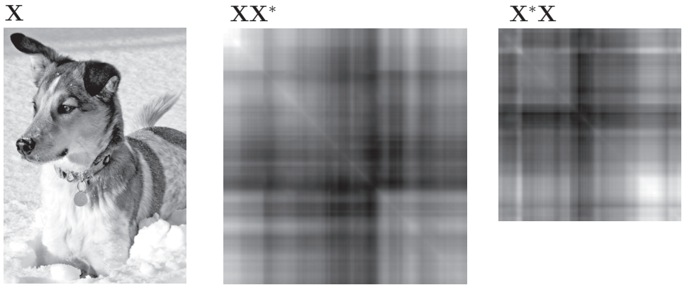
Figure 1.5 Correlation matrices XX^* and X^*X for a matrix X obtained from an image of a dog. Note that both correlation matrices are symmetric.
